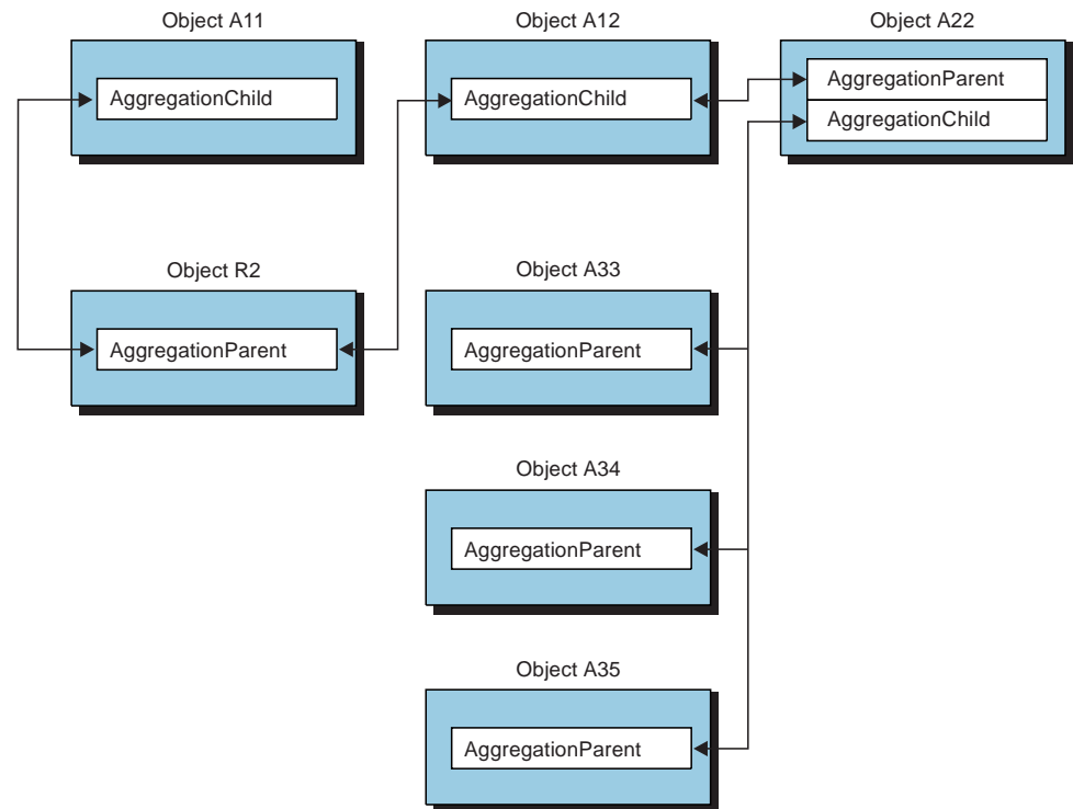
Figure 32. Links Between AggregationChild and AggregationParent Fields
