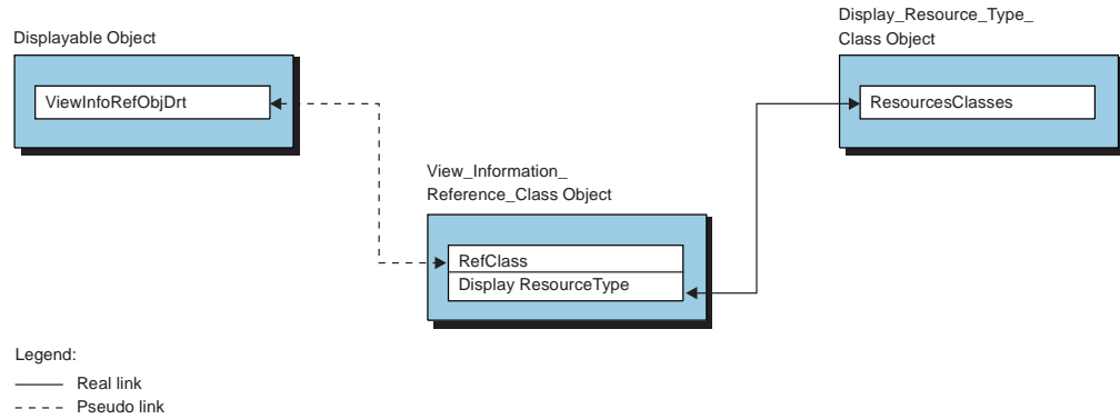
Figure 22. Second Technique for Linking Display_Resource_Type_Class Objects
