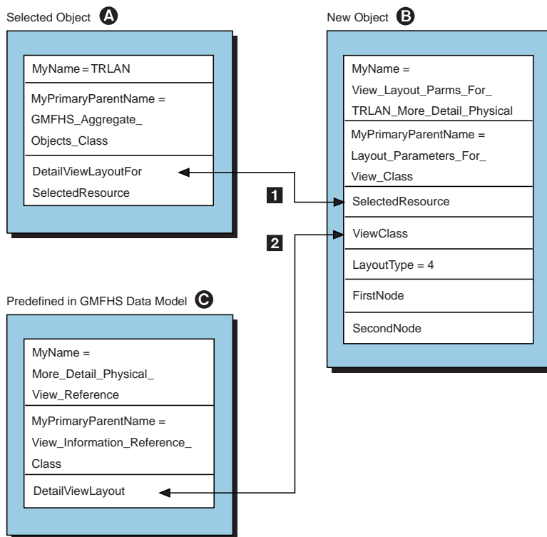
Figure 14. Defining Layout Parameters for More Detail Views
