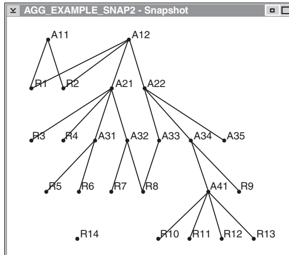
Figure 31. Aggregation Example Using Real (R) and Aggregate (A) Objects
